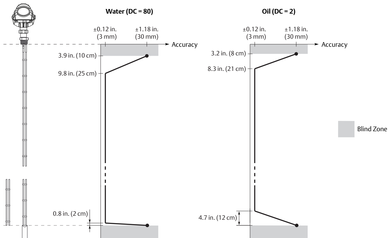
Figure 3. Accuracy Over Measuring Range for Twin Lead Probes
