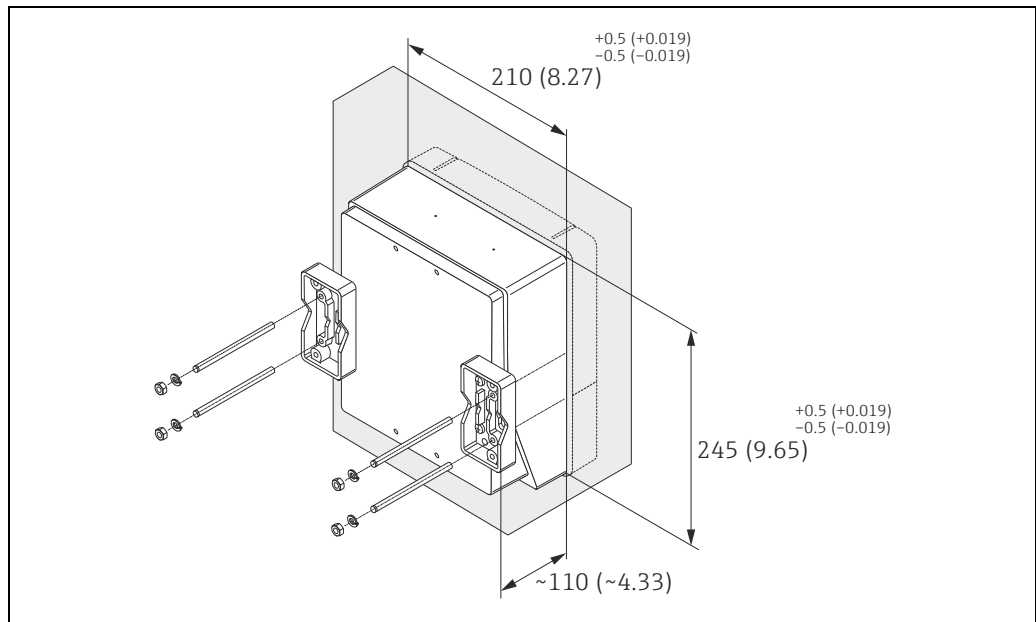
Panel-mounted installation
